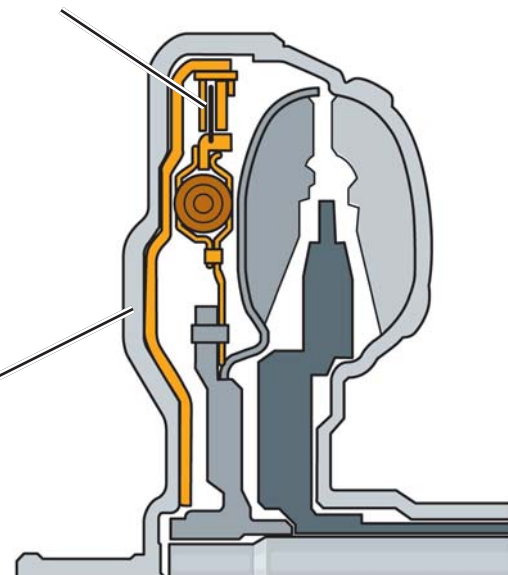
Torque Converter Lock-up Clutch
