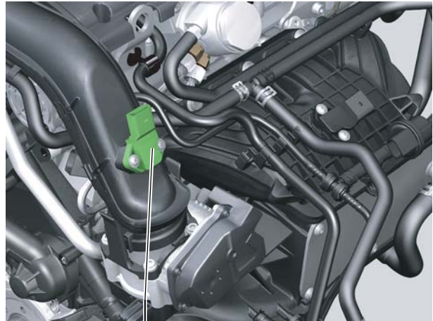
Charge air pressure sender G31 with intake air temperature sender G299 S405_042
