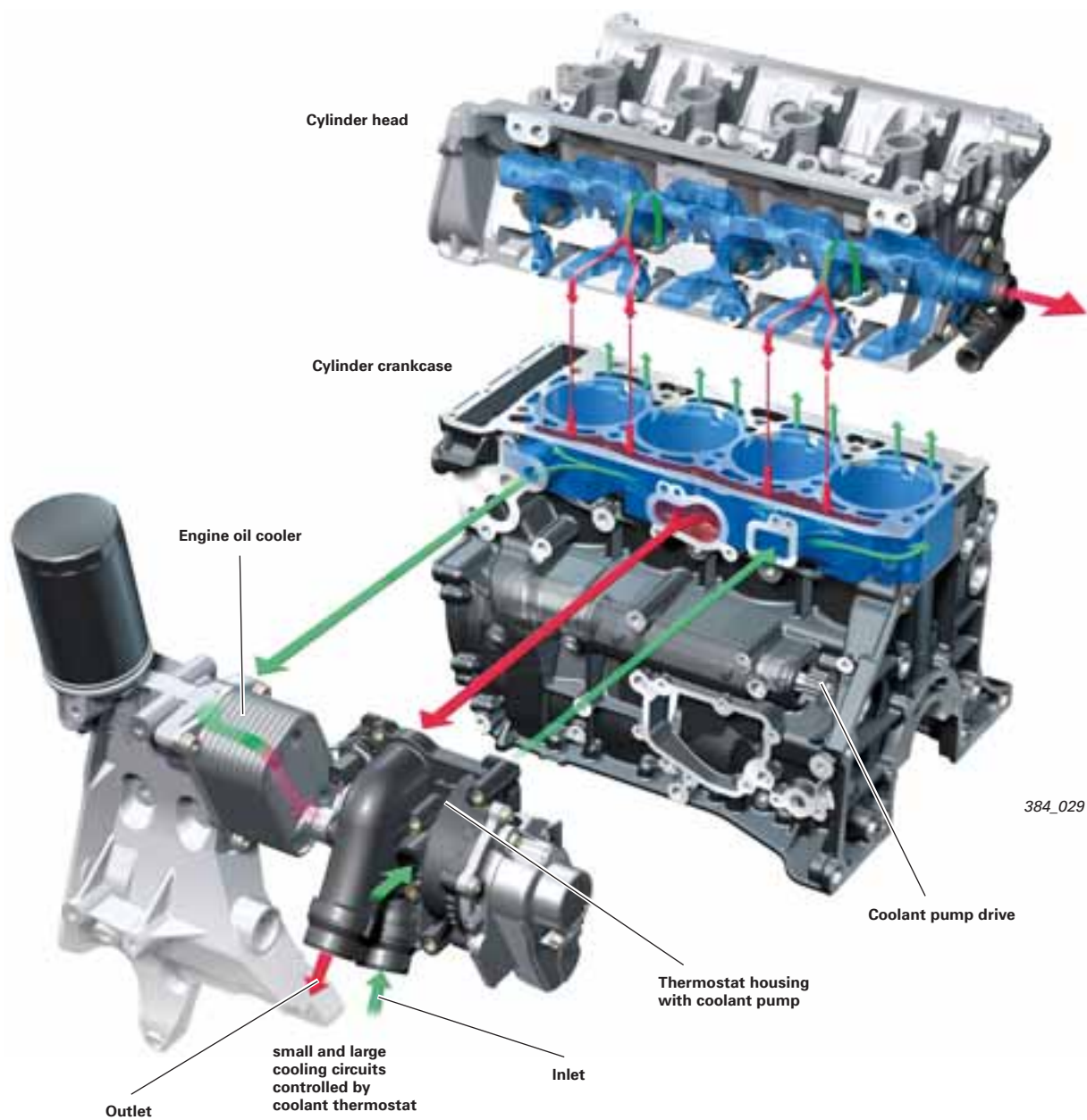
Crossflow cooling system of 1.8 litre 4V TFSI
