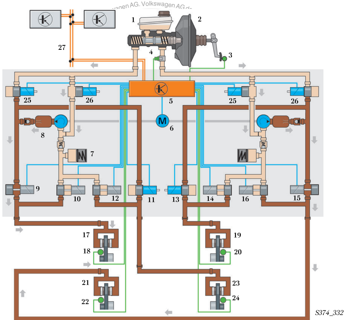
TCS hydraulic circuit diagram
