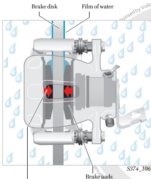
Brief application of the brake pads onto the brake disks
