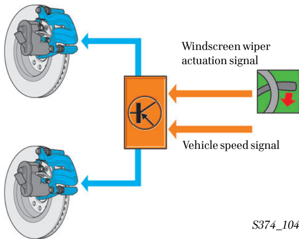
Pressure build-up at the front wheels
