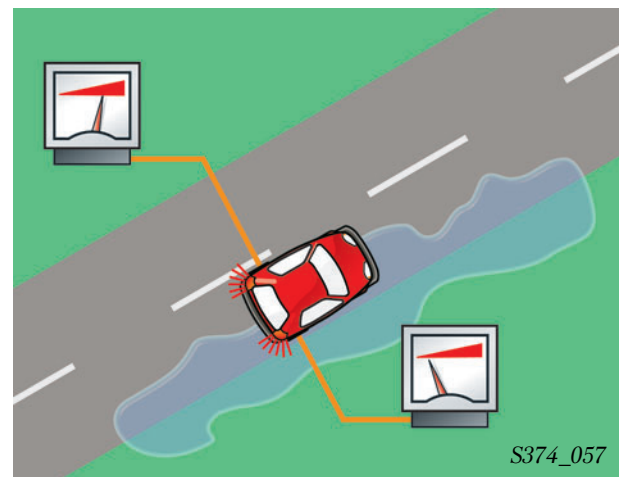
Different brake pressure distribution between the two rear wheels due to different road surface conditions
