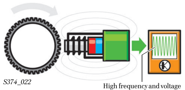
Sensor signal at high speed
