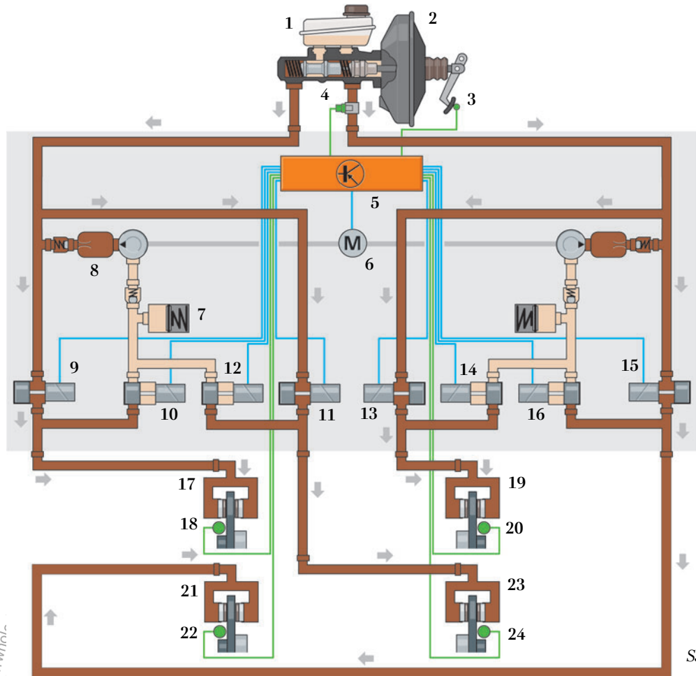
ABS hydraulic circuit diagram
