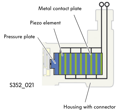
Piezo actuator (schematics)
