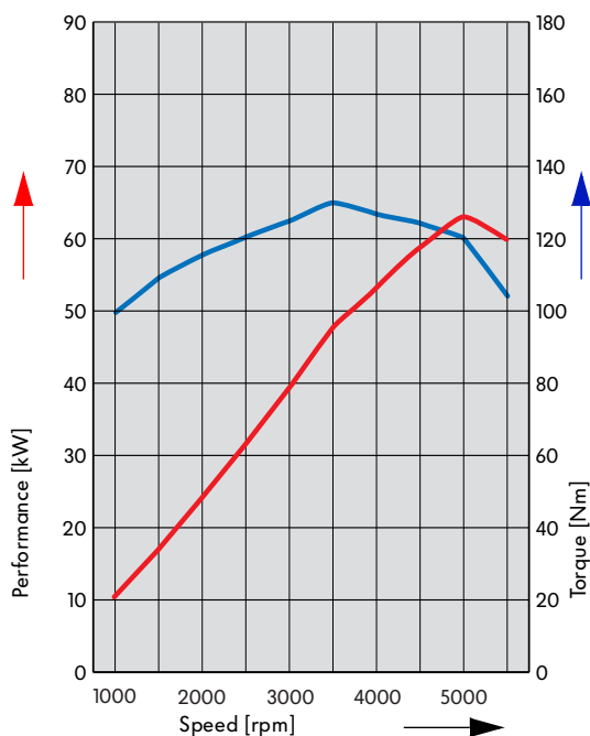
1.4 ltr./63 kW FSI engine
