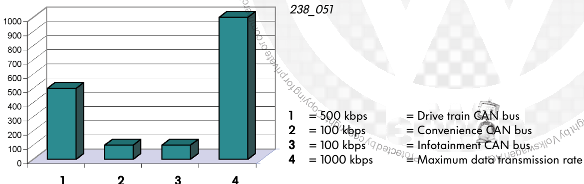
Data transmission rates on the CAN bus system
