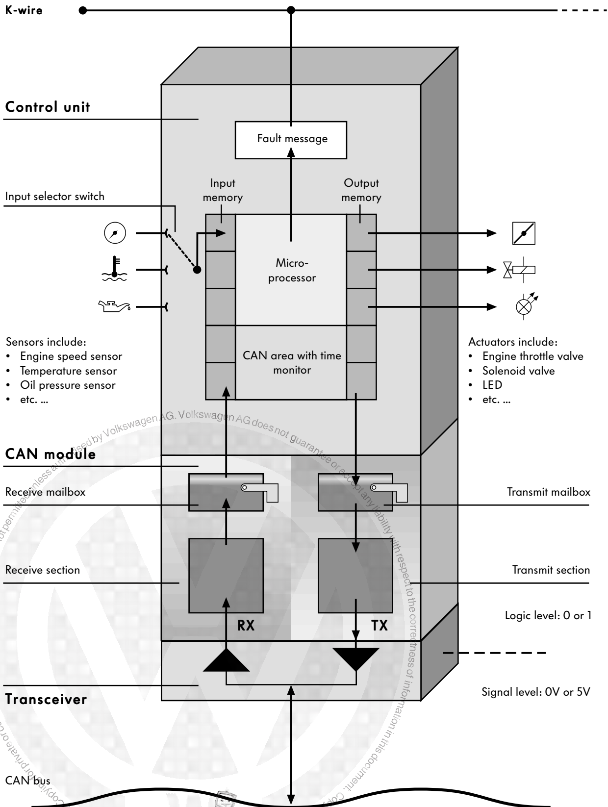
Functional unit: control unit, CAN module and transceiver
