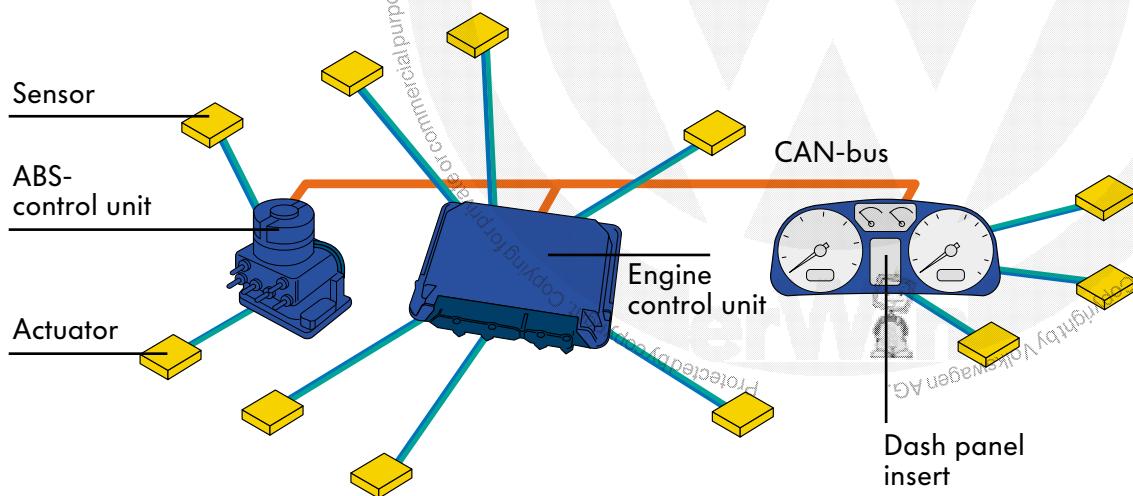
Drive train CAN network with 3 control units
