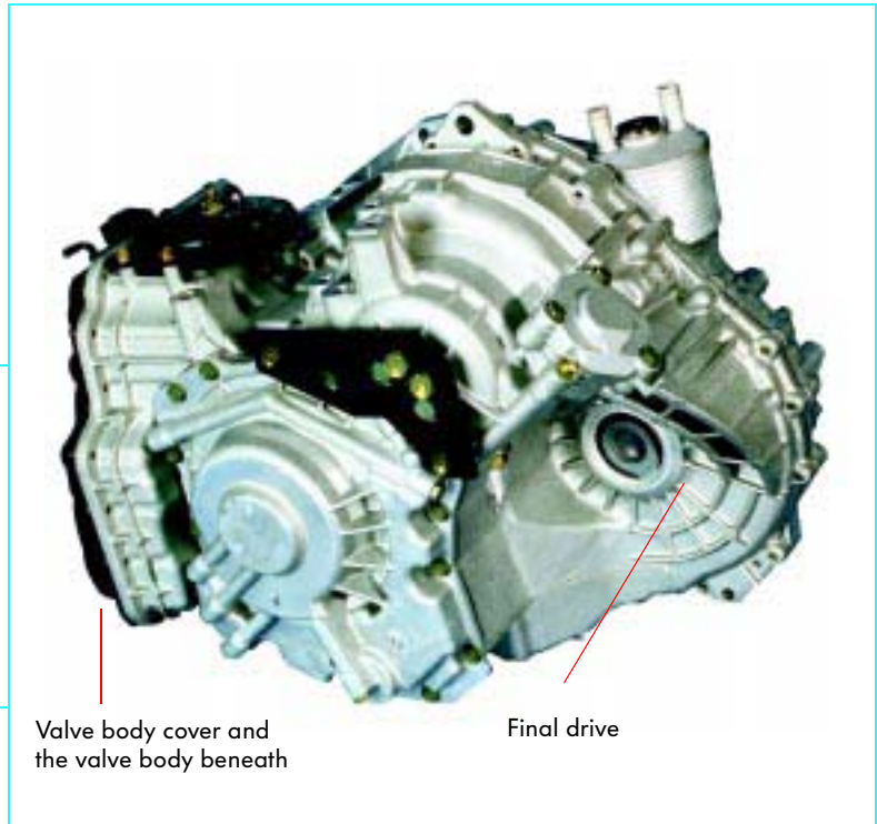
Automatic gearbox
