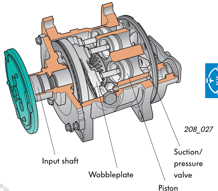
Wobbleplate compressor (non-self-regulating) Angle of wobbleplate constant Displacement constant
