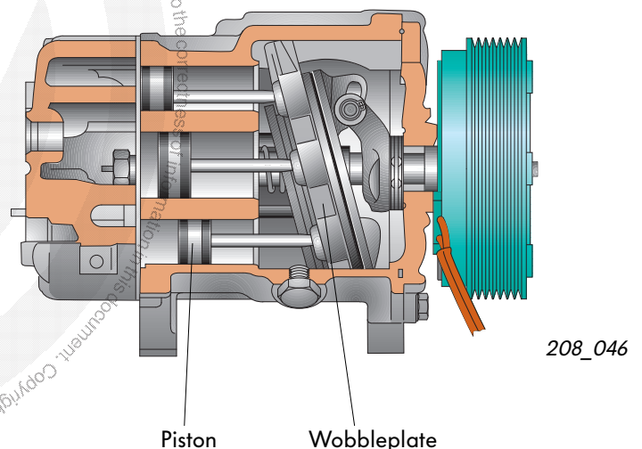
Wobbleplate compressor (self-regulating) Angle of wobbleplate variable Displacement variable
