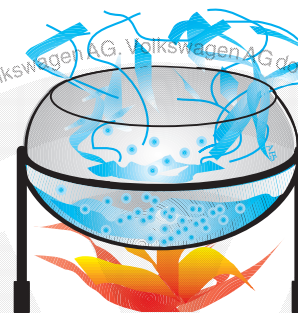
Water – becomes a gas when it absorbs heat
