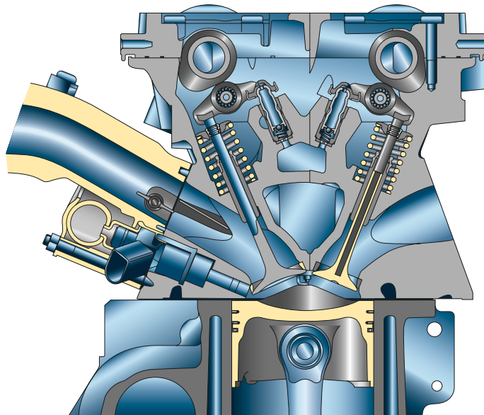
2.0L 4V-TFSI
