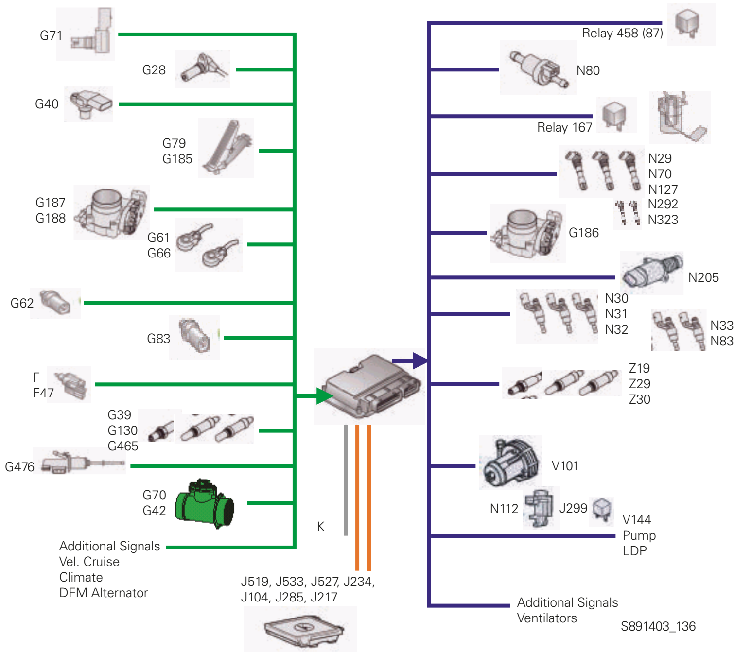
Engine Control System–Input/Output Diagram
