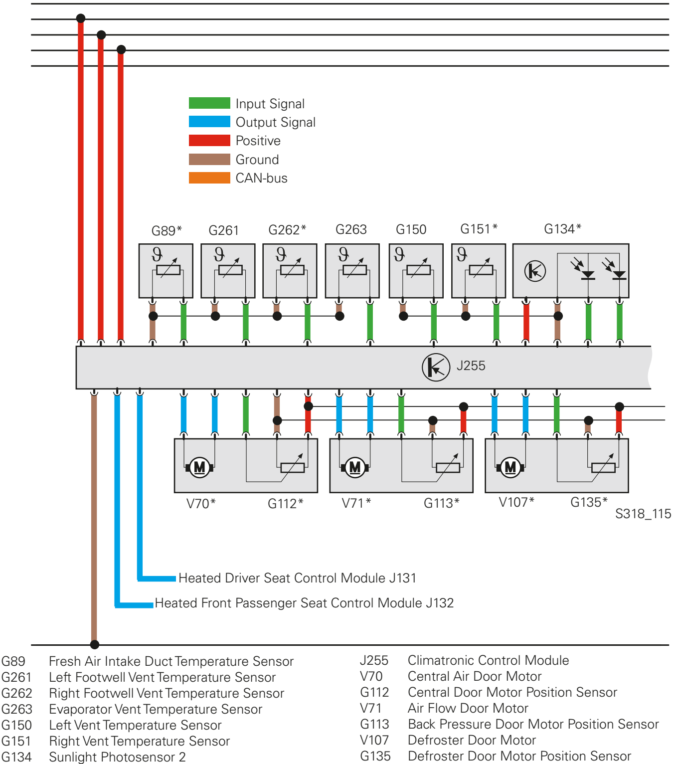
Function Diagram - Air Conditioning Systems
