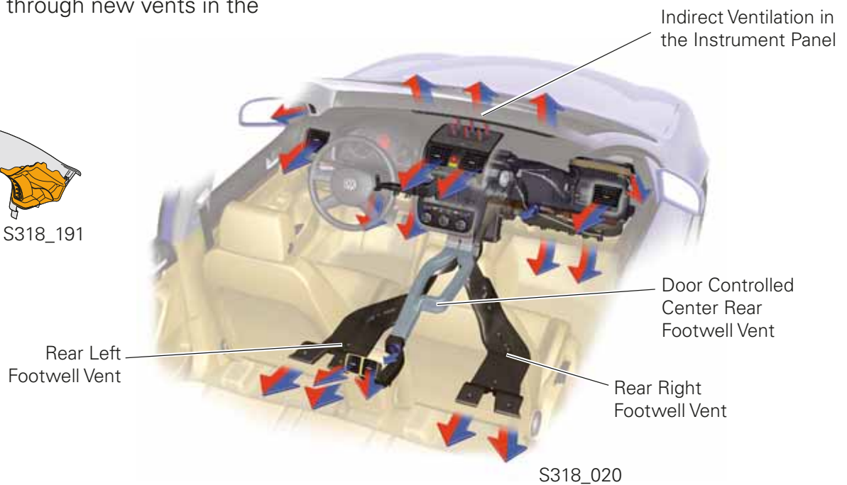
Vents in the A-Pillar
