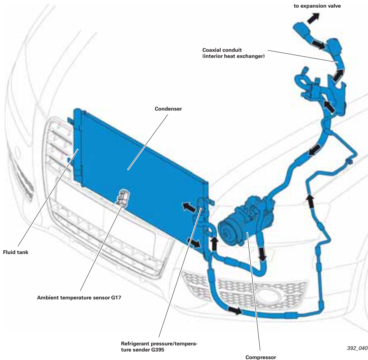
Refrigerant system in overview
