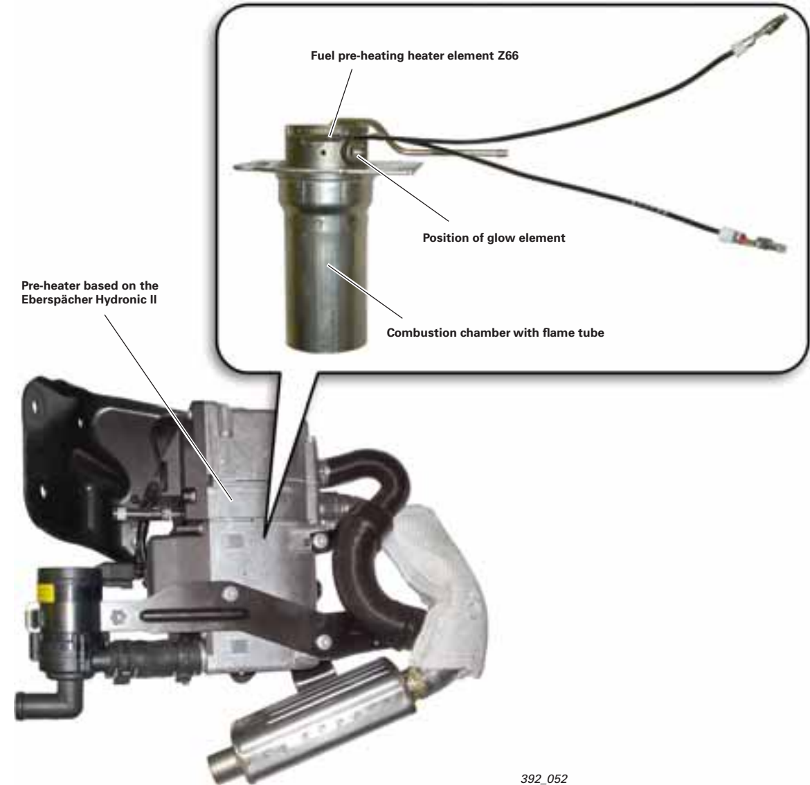
Pre-heater, optional
