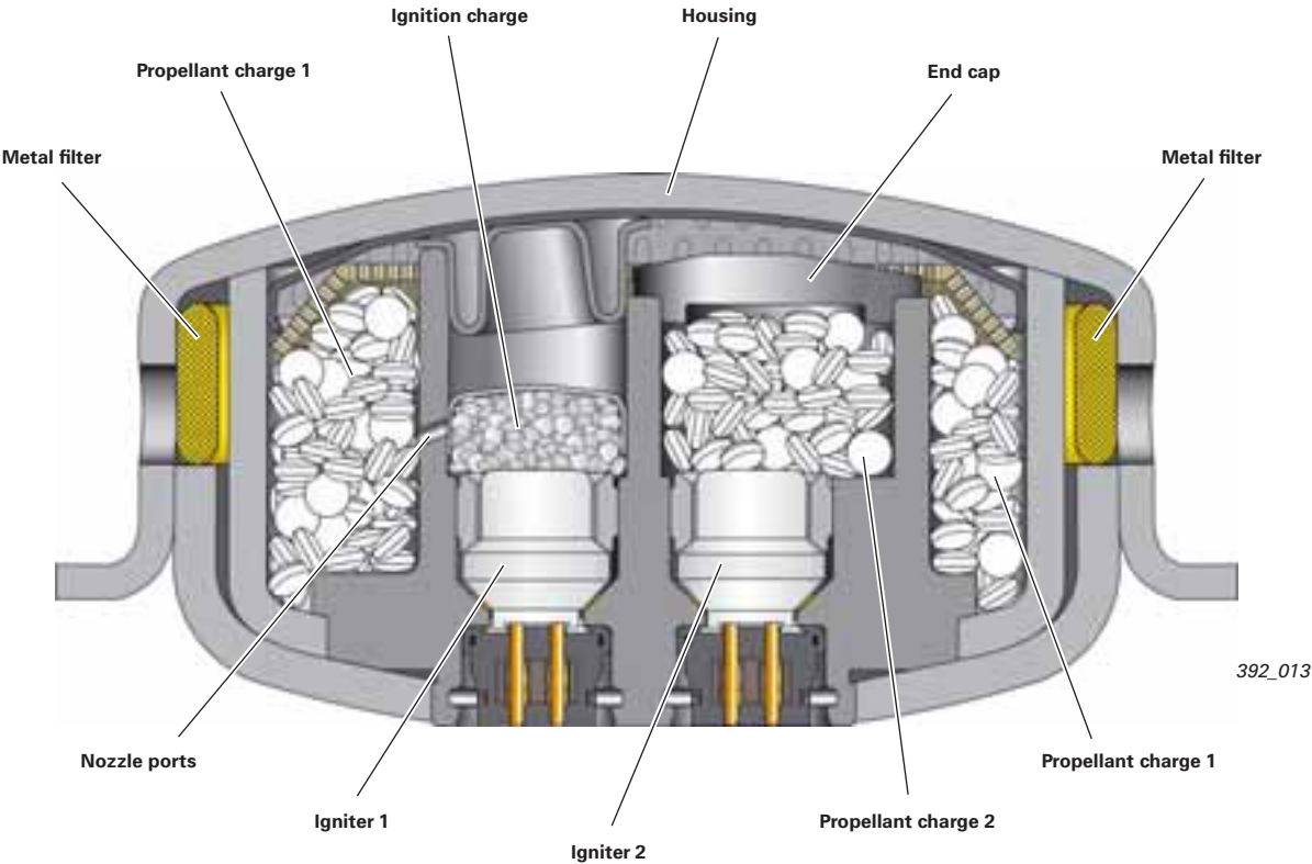
Schematic diagram of the gas generator
