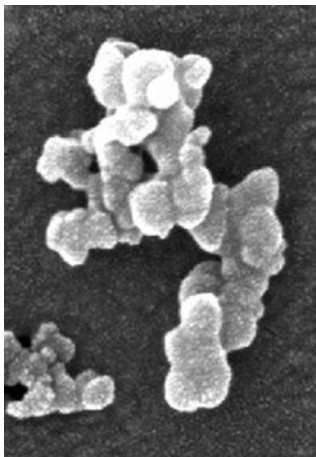
Typical particle of soot caused from diesel engine combustion
