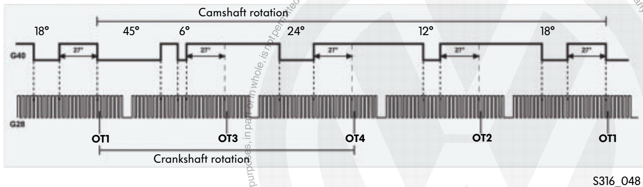
Signal pattern of Hall sender G40 (camshaft) and engine speed sender G28 during emergency running
