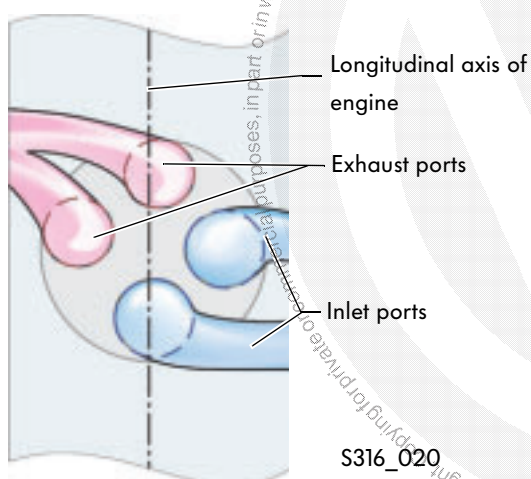
Valve pattern rotated by 45^\circ
